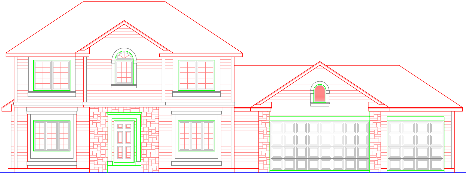
FRONT ELEVATION
